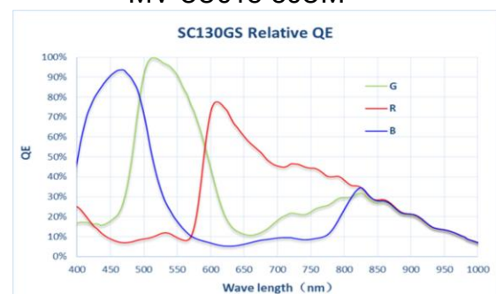
MV-CU013-80UC
