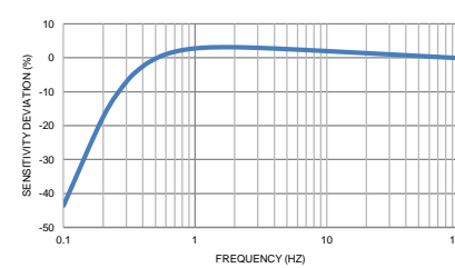
TYPICAL LOW FREQUENCY RESPONSE
