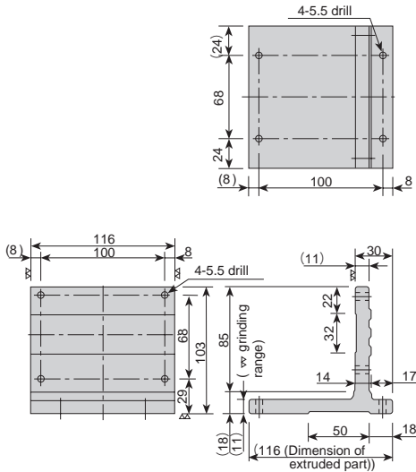
[BA31-BK-L01] Material: Aluminum alloy, mass 2.1 kg
