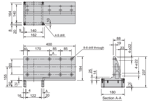
[BA1T7-BK-L03] Material: Aluminum alloy, mass 0.8 kg
