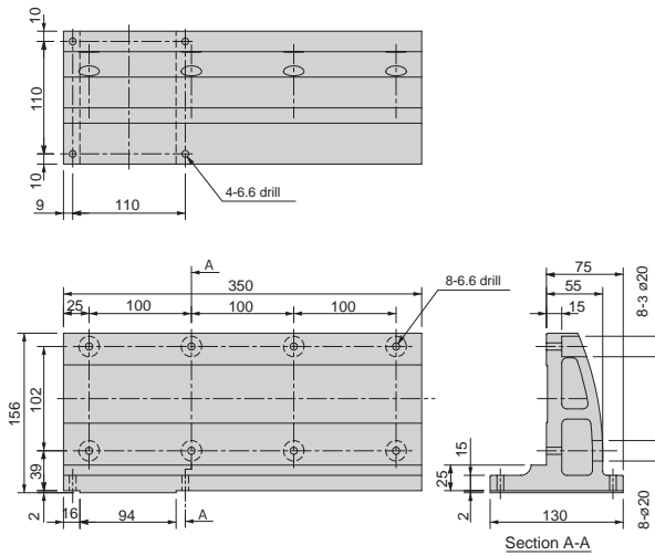
[BAT7T5-BK-L03] Material: Aluminum alloy, mass 0.5 kg
