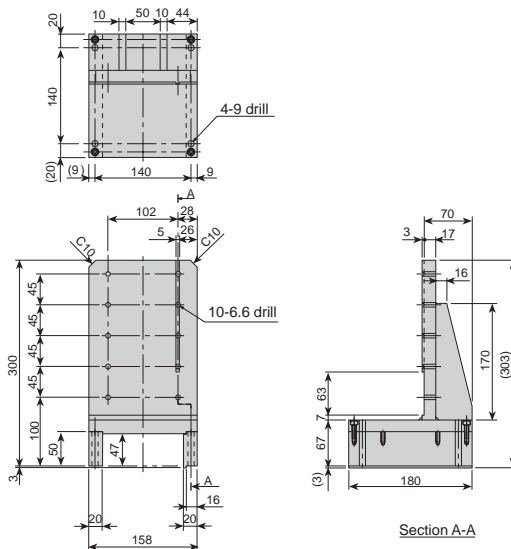
[BA53-BK-L01] Material: Aluminum alloy, mass 4.5 kg
