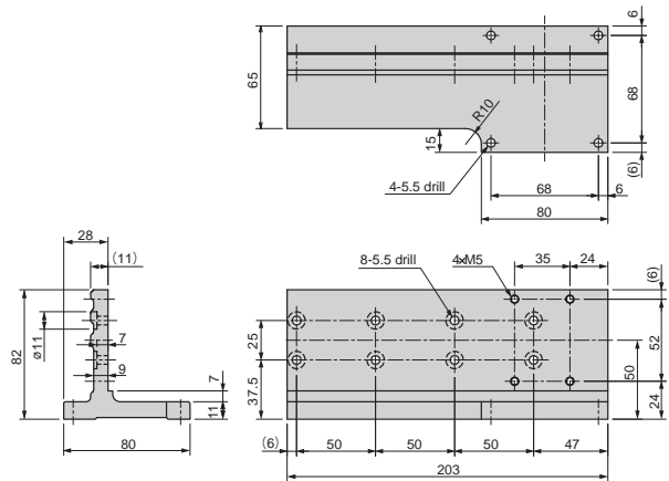
[BA10-BK-L03] Material: Aluminum alloy, mass 0.9 kg
