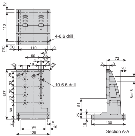
[BA31-BK-L01] Material: Aluminum alloy, mass 2.1 kg
