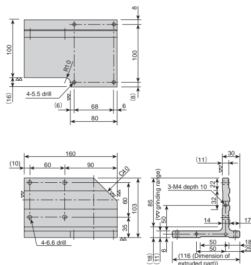
[BA10-BK-L03] Material: Aluminum alloy, mass 0.9 kg
