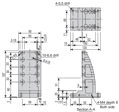
[BA53-BK-L01] Material: Aluminum alloy, mass 4.5 kg
