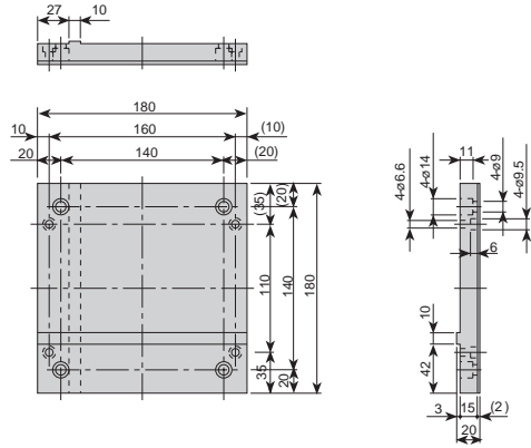
[BA11-BK-L01] Material: Aluminum alloy, mass 1.8 kg
