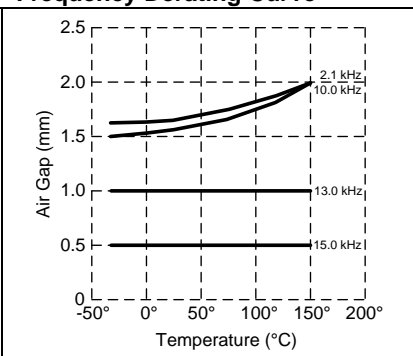
Figure 3. Temperature Air Gap Frequency Derating Curve
