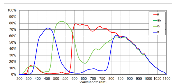
MV-CH100-60UC
