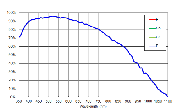
MV-CH100-60UM
