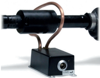
Ring stator for inductive supply
