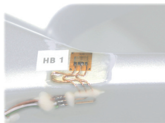
Strain gauge applications & calibration, e.g., according to VDI/VDE 2646
