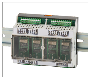
4-channel hat rail version
