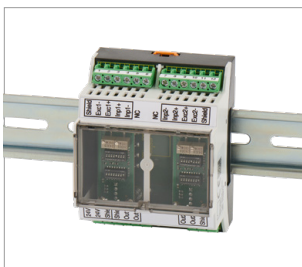
2-channel hat rail version
