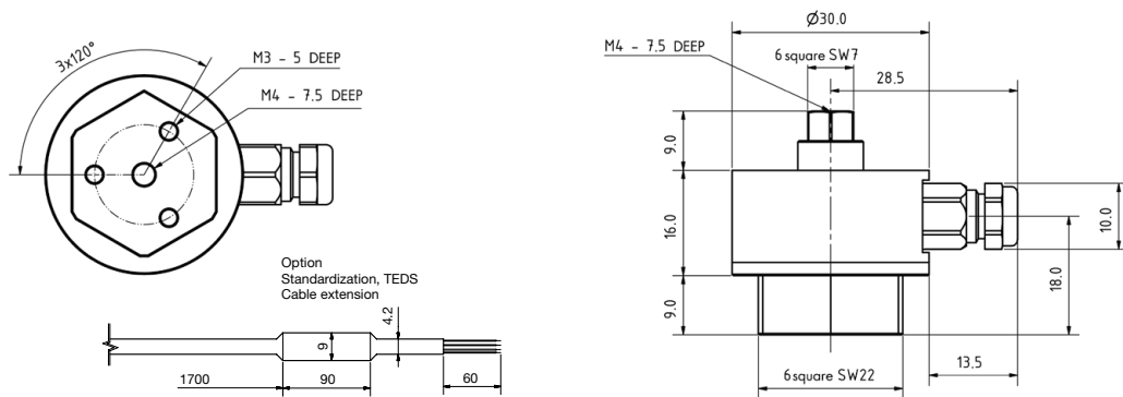
Dimensional drawing 1 – Measuring ranges from 0 ... ±20 N up to 0 ... ±200 N | from 0 ... ±4.5 lbs up to 0 ... ±45.0 lbs
