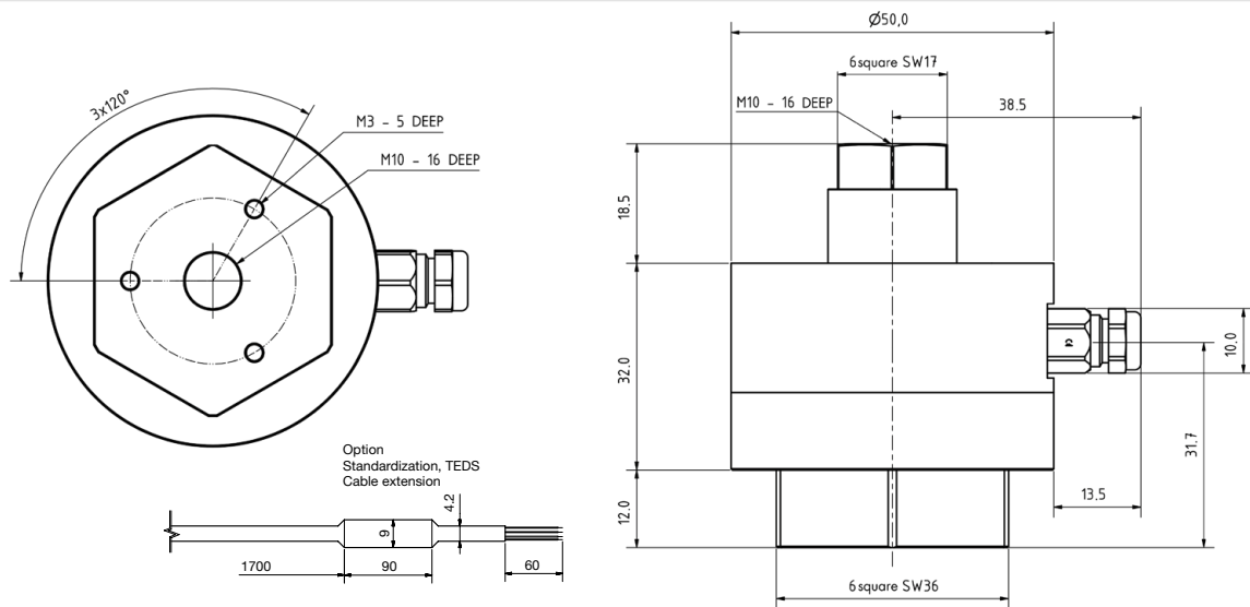
Dimensional drawing 2 – Measuring ranges from 0 ... ±500 N up to 0 ... 10 kN | from 0 ... ±112.4 lbs up to 0 ... ±2.2 klbs
