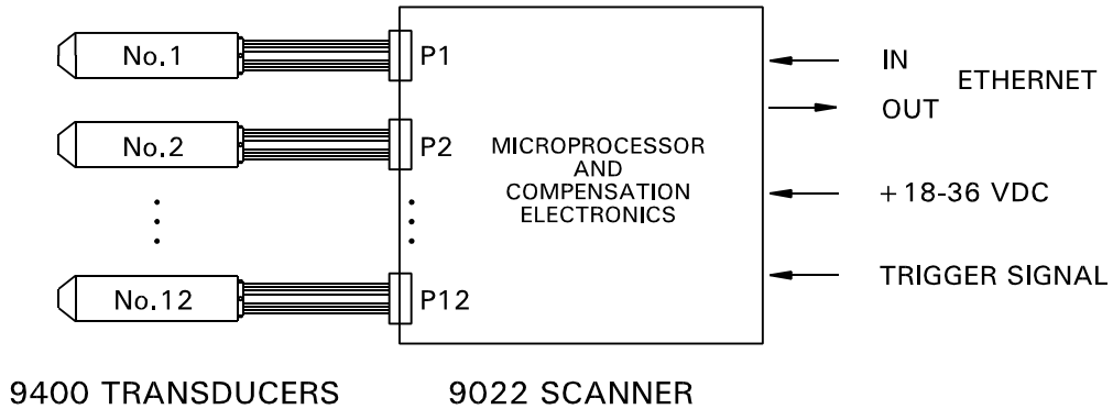
All-Media Intelligent Pressure Scanner Functional Diagram
