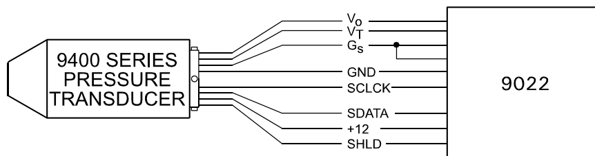
9400 CONNECTION TO 9022
