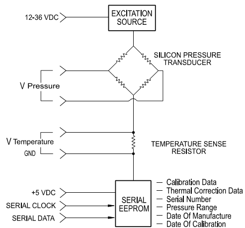
Electrical Block Diagram
