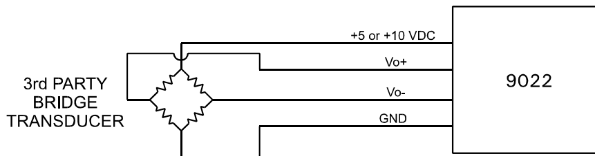
BRIDGE TRANSDUCER CONNECTION TO 9022
