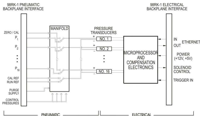
Pneumatic Intelligent Pressure Scanner Functional Diagram
