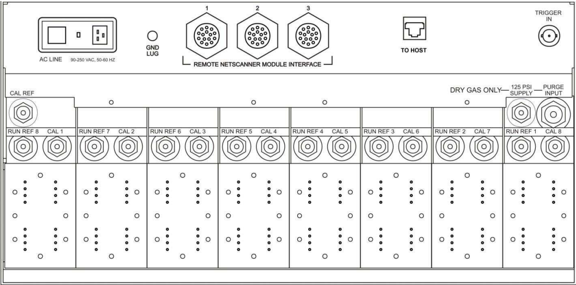
98RK-1 Scanner Interface Rack Rear Panel Layout
